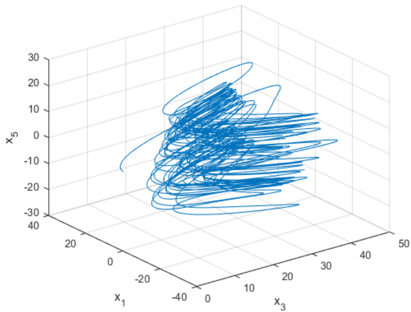
(g) 3-D Projection of the 5D hyperchaotic Lorenz system on (x_3, x_1, x_5)
